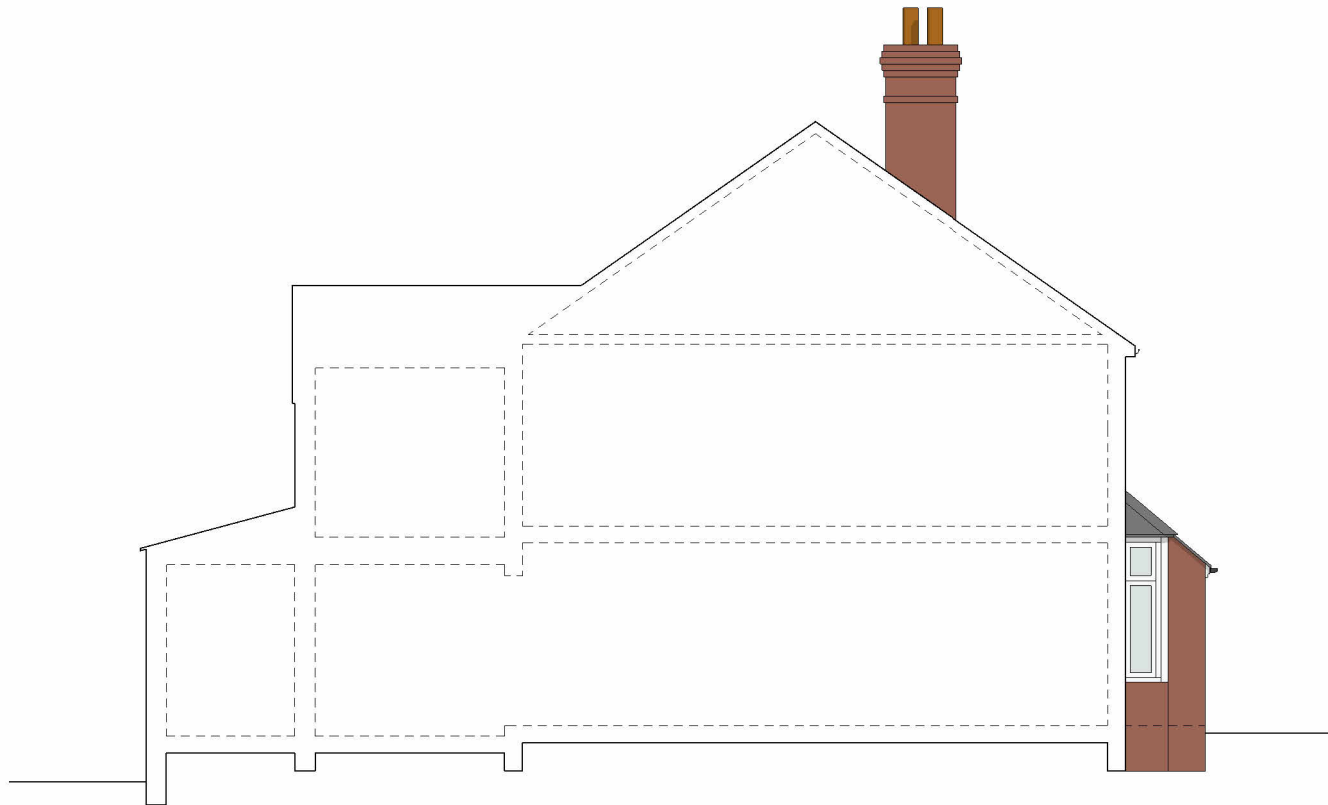
4 Existing West Elevation A2.00 1 : 100
