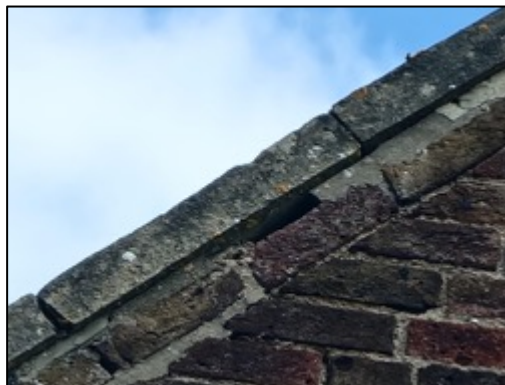
Figure 28 – Gaps under stone coping where mortar is missing.
