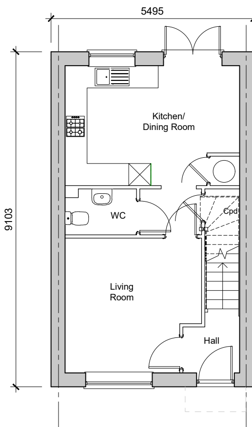
Ground Floor Plan 2-Bedroom House 79.13sqm / 851.80sqft GIA (as shown) Plots - 31, 32 Handed - 33
