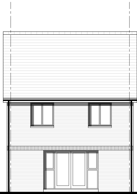
Rear Elevation
