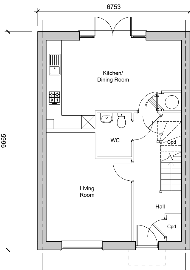
Ground Floor Plan 4-Bedroom House 105.88sqm / 1150.40sqft GIA (to finished) Plot - 48 Handed - 49
