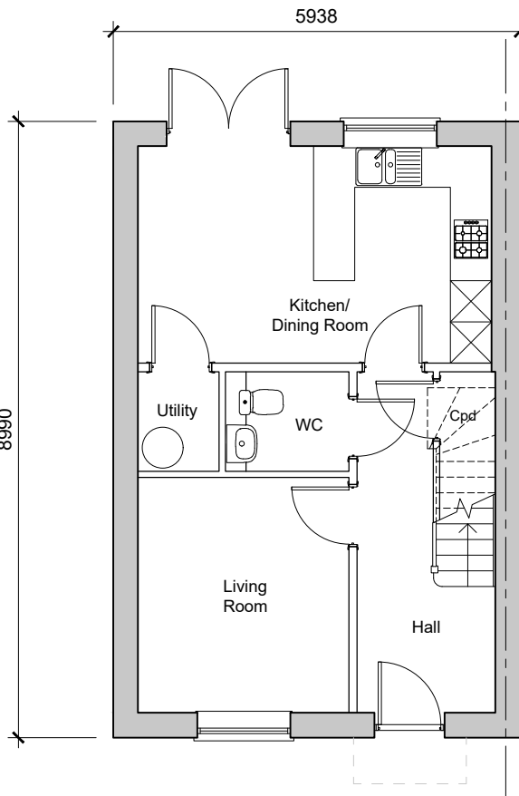
Ground Floor Plan 3-Bedroom House 88.00sqm / 925.69sqft GIA (to include) Plots - 5, 10, 12, 14, 28, 29, 34, 35, 37, 46 Handed - 11, 13, 15, 16, 30, 36, 38, 47, 51, 54, 55
