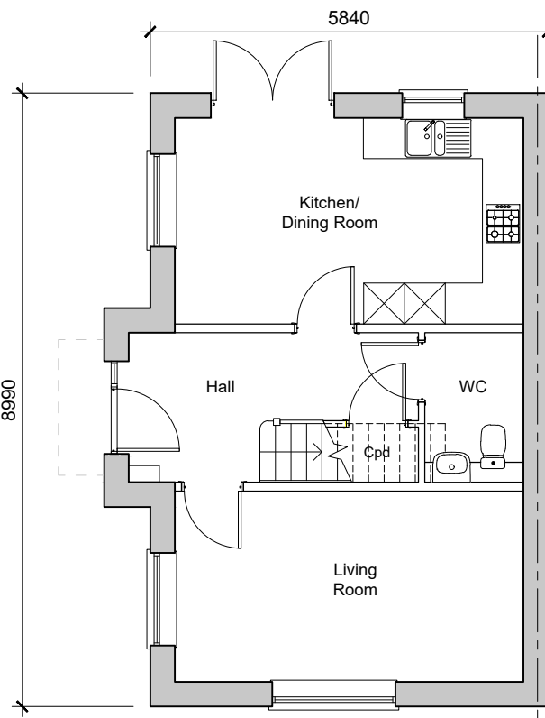
Ground Floor Plan 3-Bedroom House 87.60sqm / 942.91sqft GIA (m 2 / sqft) Plots - 9, 40, 41, 44, 45, 50, 53, 56 Handed - 6, 38, 42, 52
