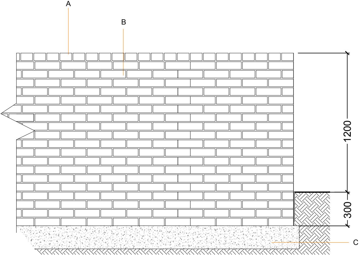
1200mm Front Elevation Scale 1:20
