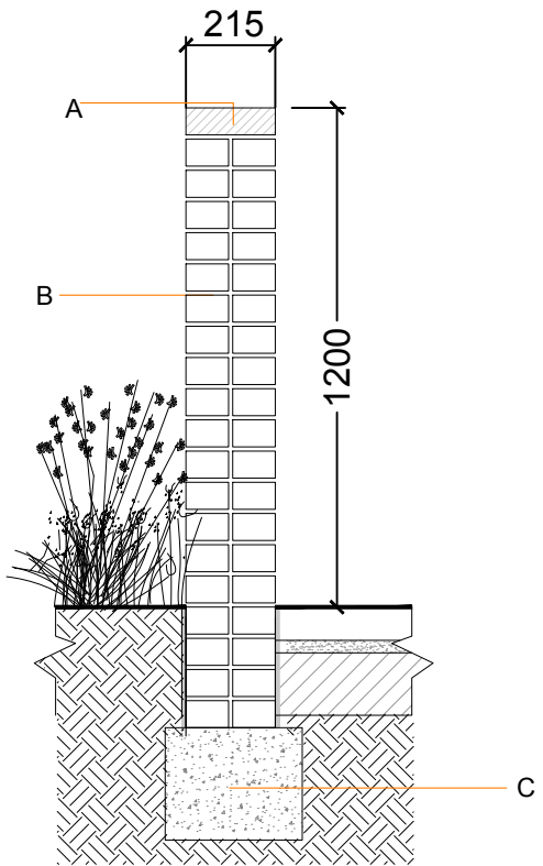
1200mm Side elevation Scale 1:20
