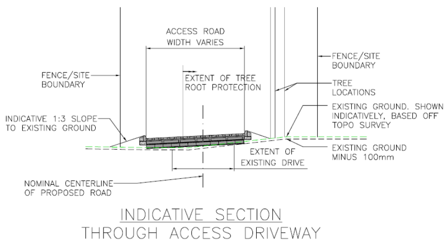
Figure 3 – Indicative section
