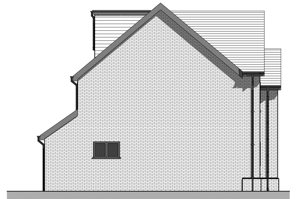
SIDE ELEVATION 1:100 Land North of Oakview, Mill Lane, Wokingham RG41 5DF
