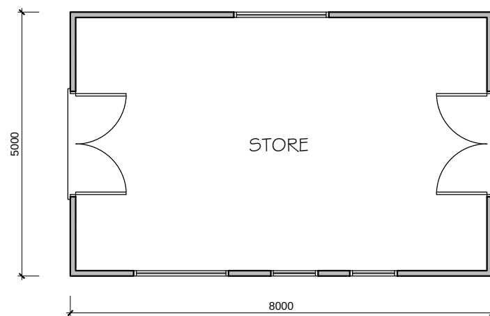
PROPOSED GROUND FLOOR SHED B - GOAT FOOD STORE Volume = 138m 3
