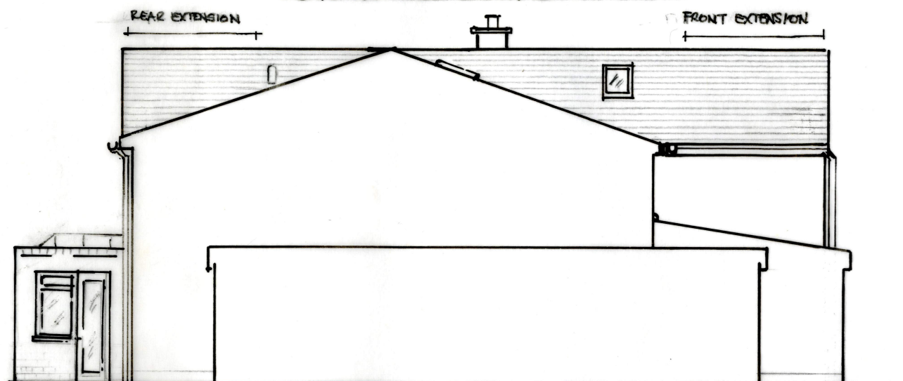
EXISTING SIDE ELEVATION TO S.W.
