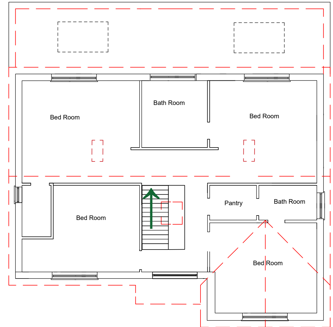
2 PROPOSED FIRST FLOOR 1:100
