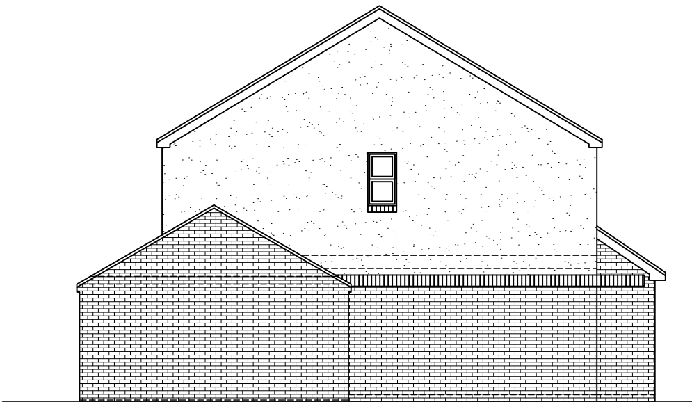
Existing Left Side Elevation Scale: 1/100
