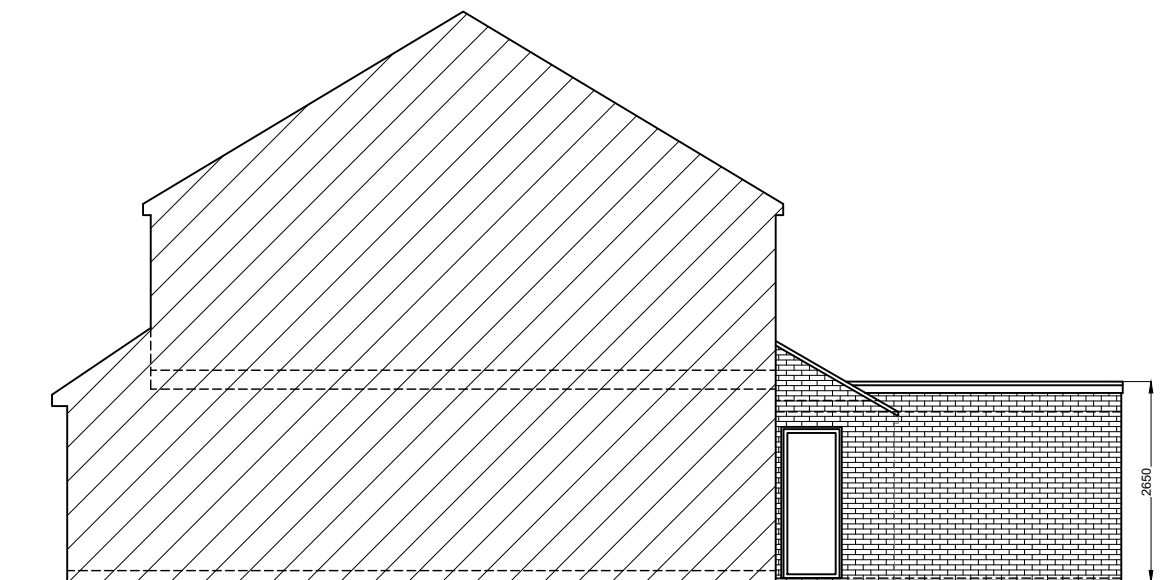
Proposed Right Side Elevation Scale: 1/100
