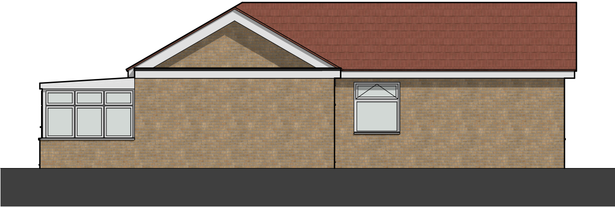
2 Side Elevation 1:100
