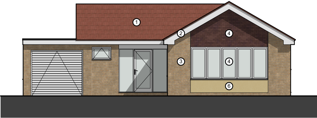
1 Front Elevation 1:100
