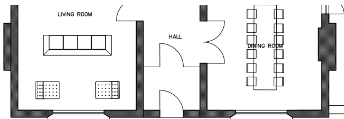
PROPOSED GROUND FLOOR PLAN 1:100
