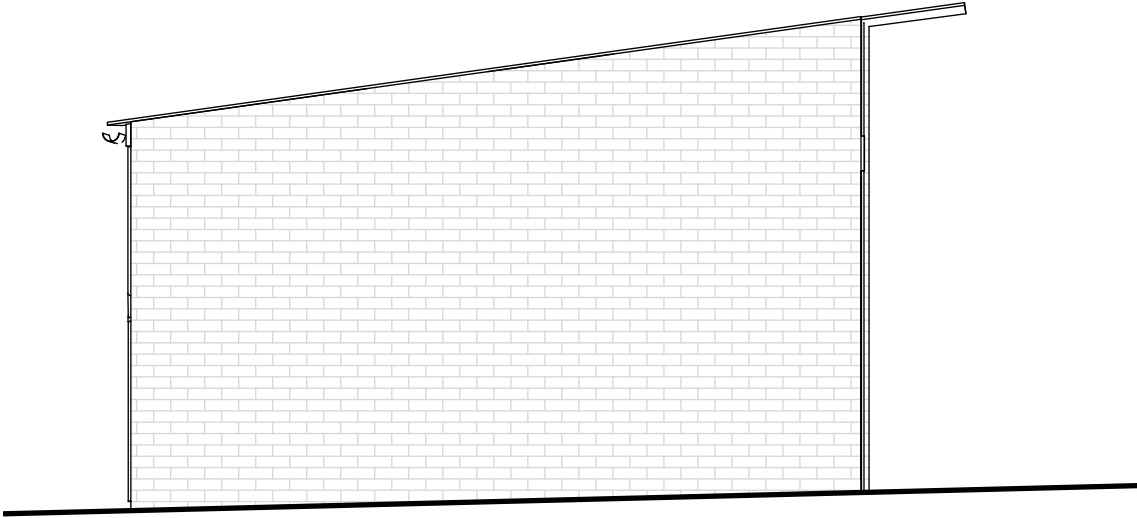
Existing Small Barn West Elevation 1 : 50
