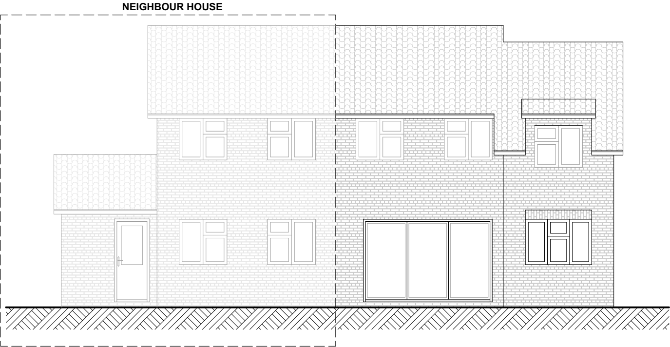
Rear elevation
