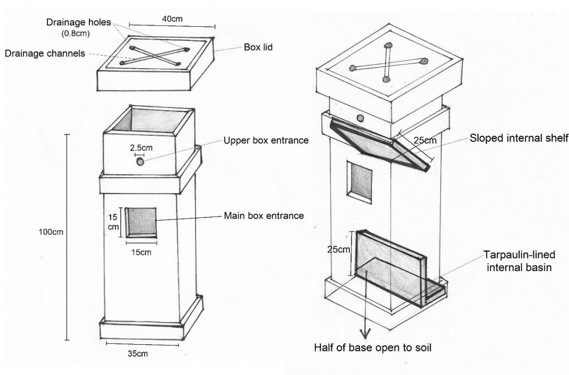
Figure 3.5. Diagrams of the wooden beetle boxes used in this study, with key features and dimensions labelled.
