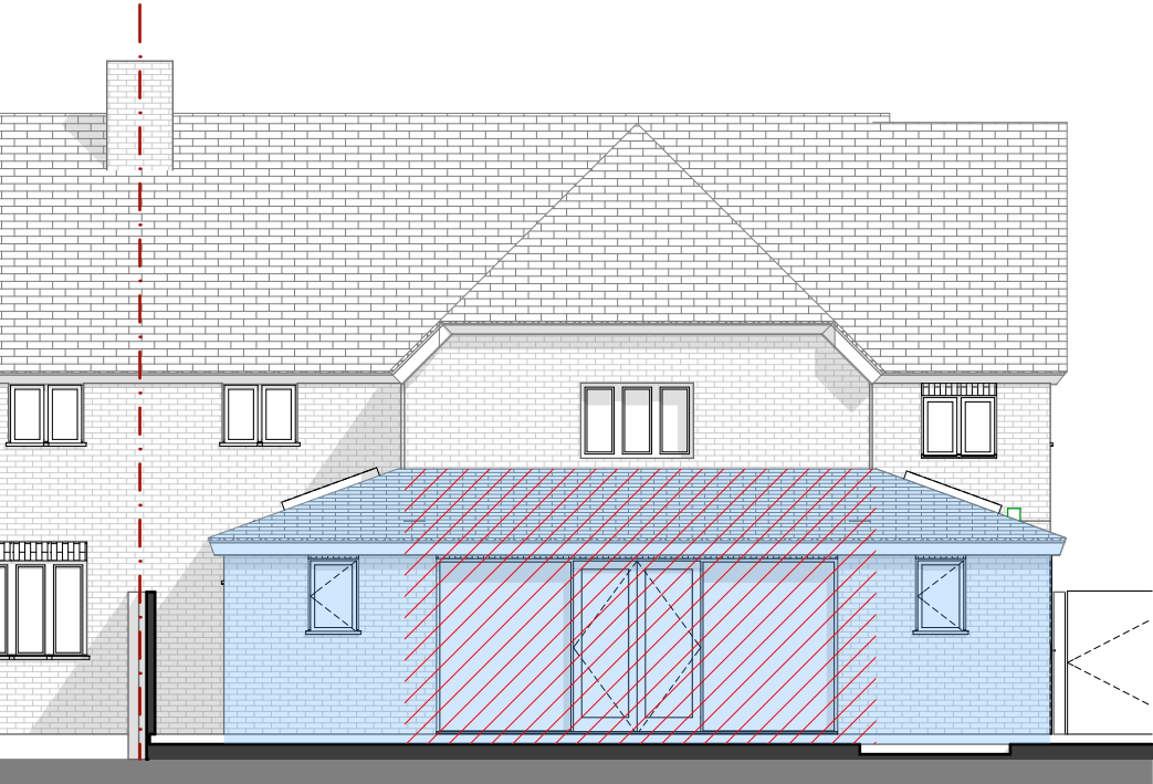
Northwest Elevation 1:100
