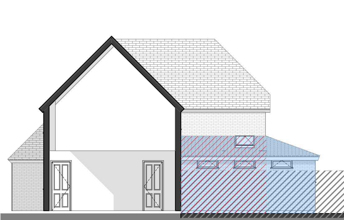
Northeast Elevation 1:100
