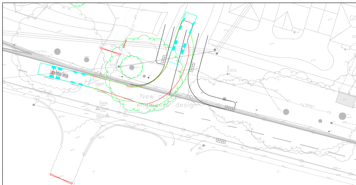
REFUSE VEHICLE TRACKING - LEFT IN
