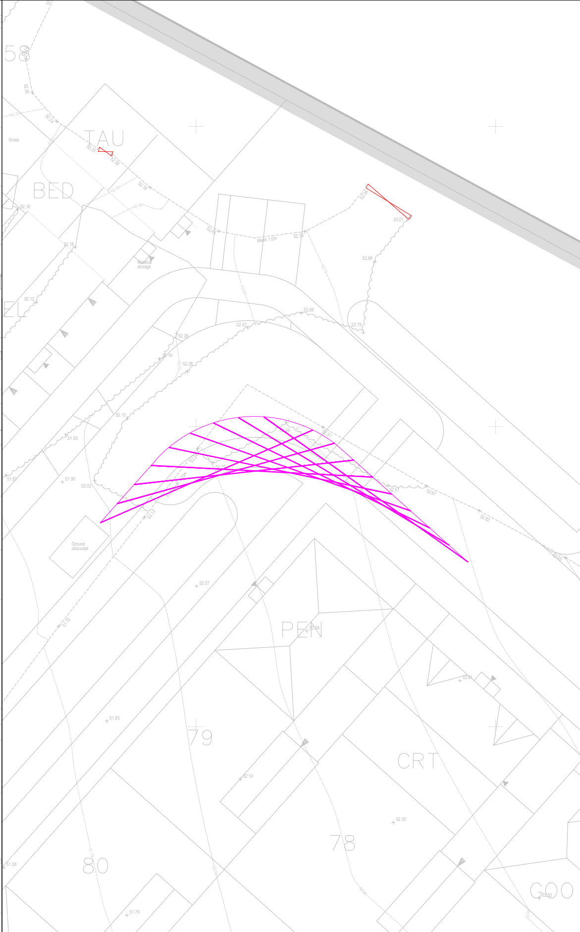
17M FORWARD VISIBILITY SPLAY - OUTSIDE PLOT 79
