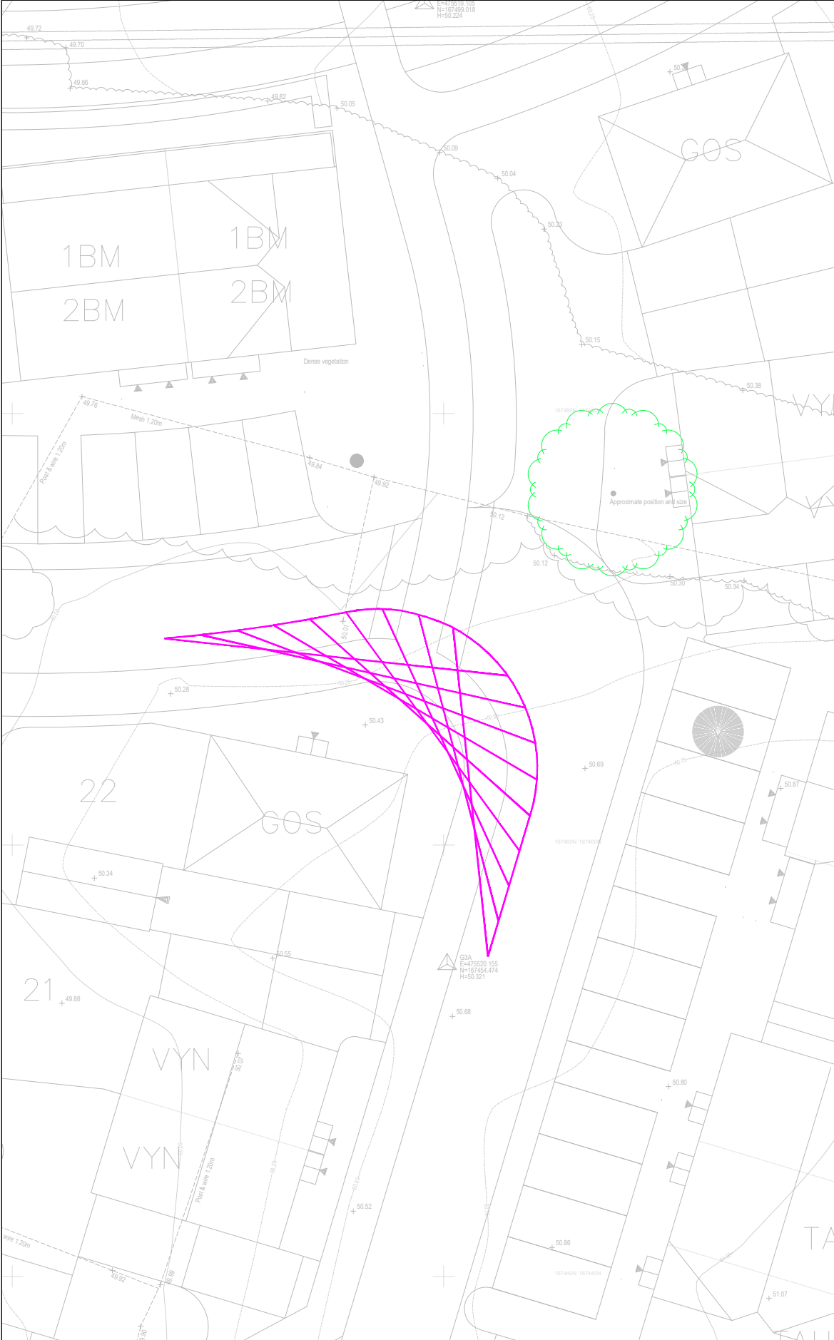
17M FORWARD VISIBILITY SPLAY - OUTSIDE PLOT 22
