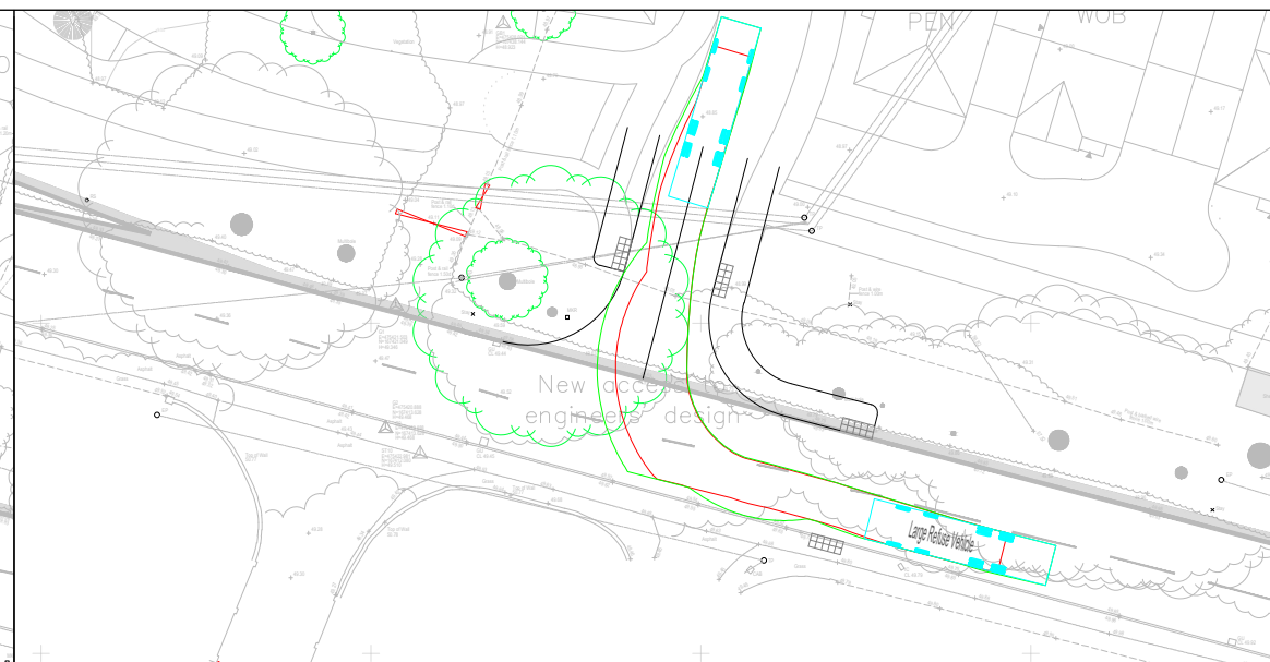
REFUSE VEHICLE TRACKING - RIGHT IN
