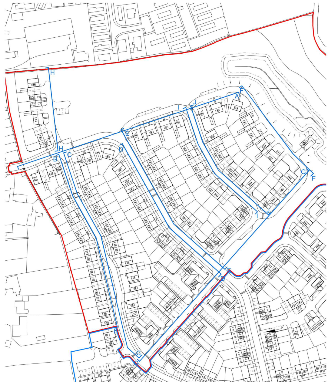
Key Plan 1:2000
