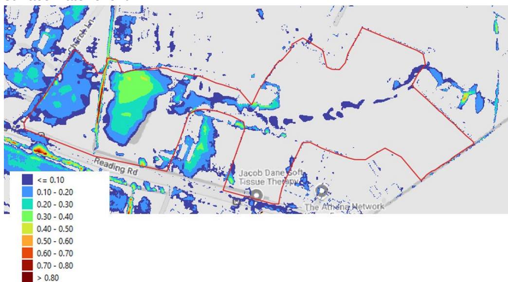
Figure 4: Extract of Surface Water Flooding Depths from ACE
