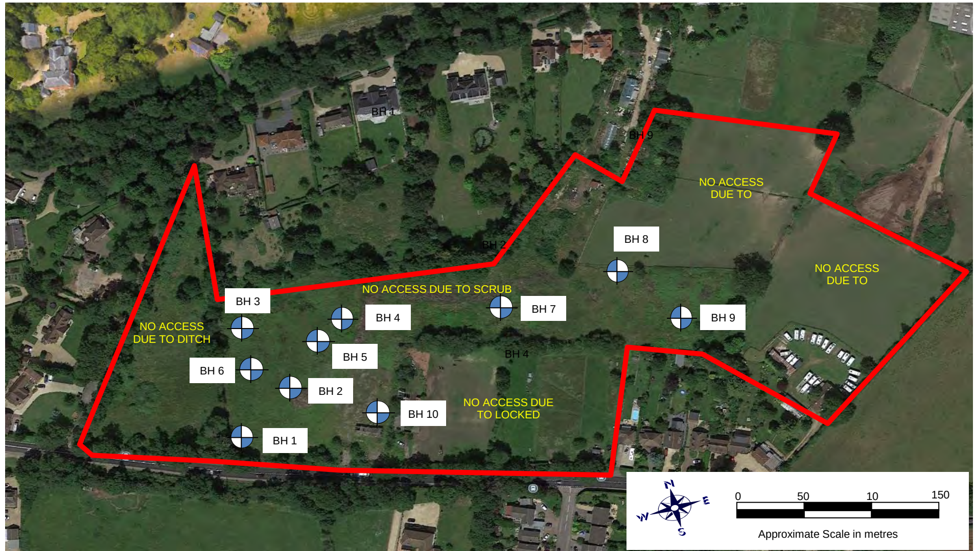
Site Plan
