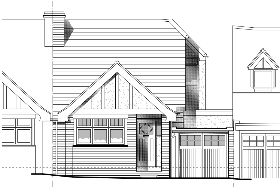
FRONT ELEVATION 1:100
