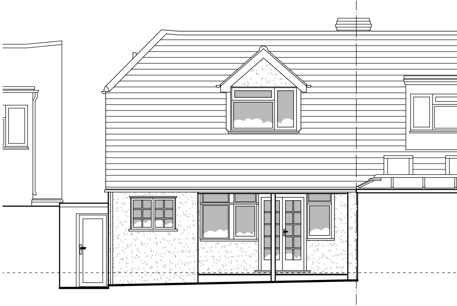
REAR ELEVATION 1:100
