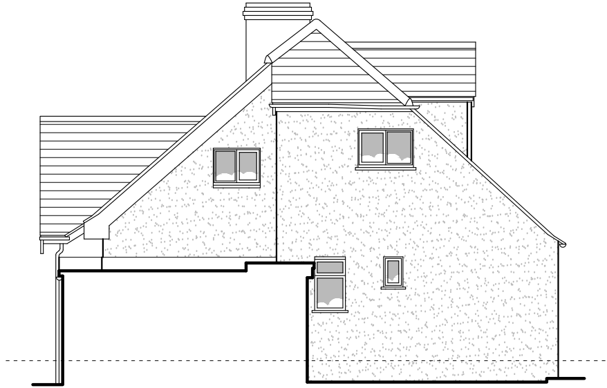
SIDE ELEVATION 1:100
