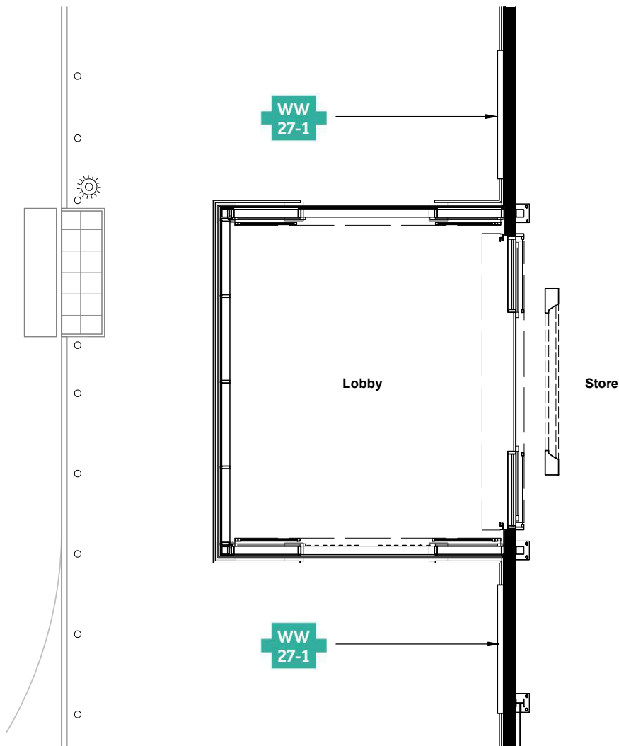
1 Welcome Wall Location Plan 1 : 100
