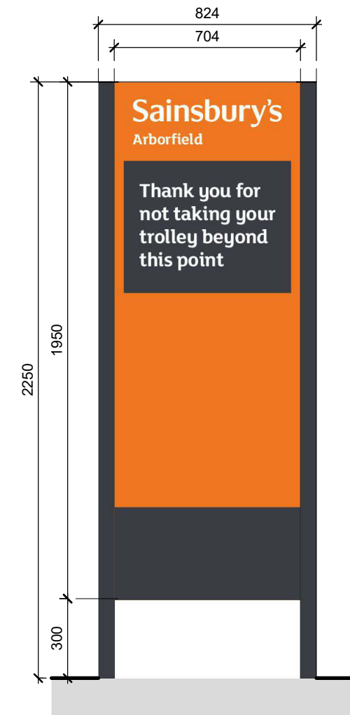
5 2.25m Pedestrian Totem - Rear 1:20
