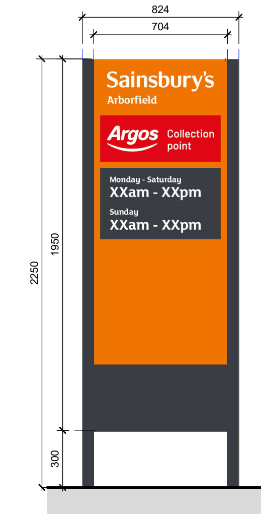
4 2.25m Pedestrian Totem - Front 1:20
