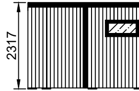
Rear Elevation
