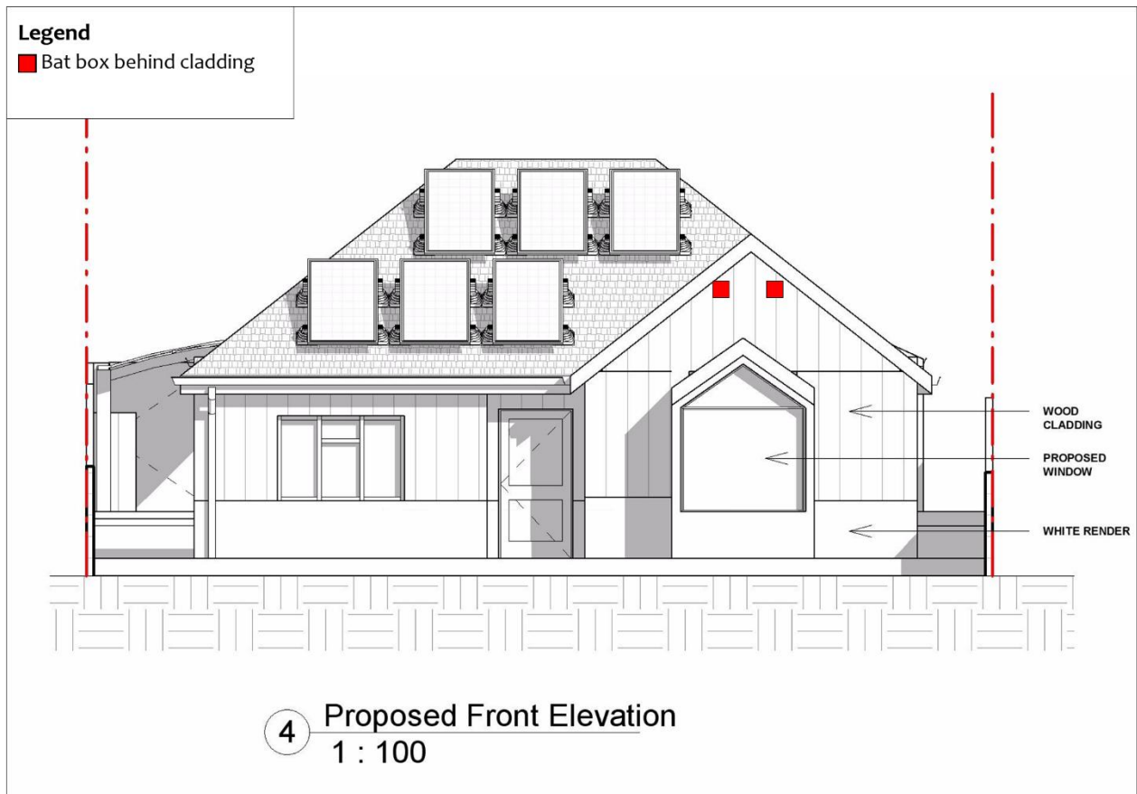
Figure 4 – Proposed front elevation showing locations of bat mitigation measures
