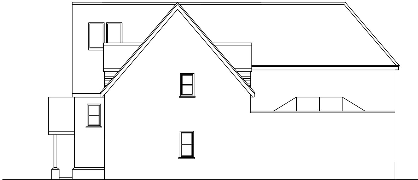
Proposed SE Elevation
