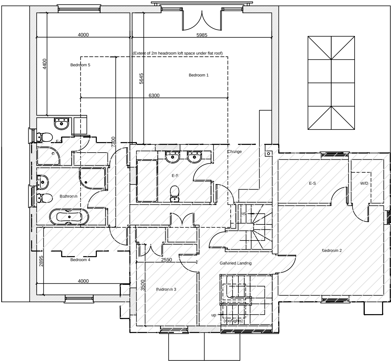
Proposed First Floor (Existing areas shaded)
