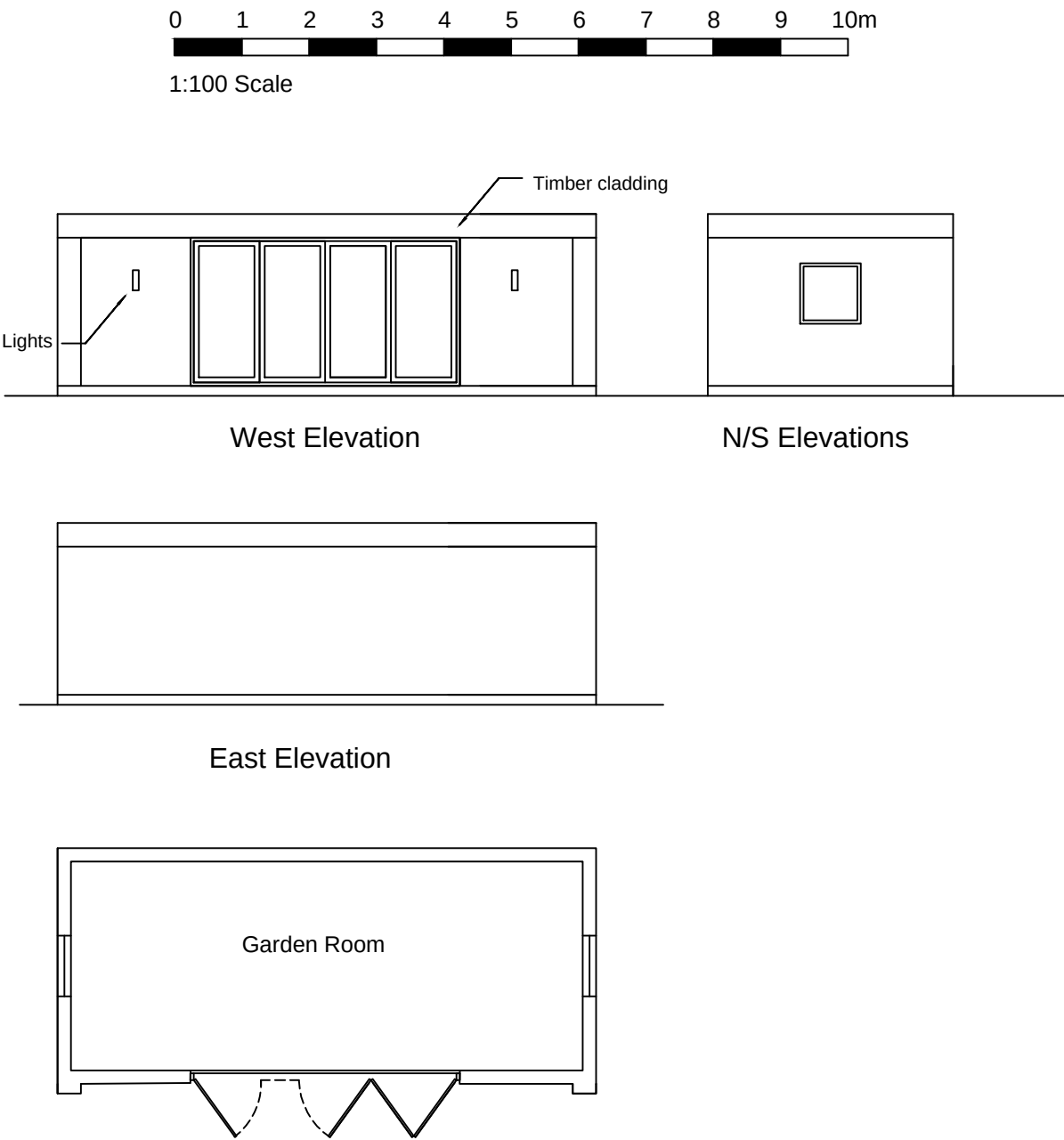
Plan and Elevations of Garden Room
