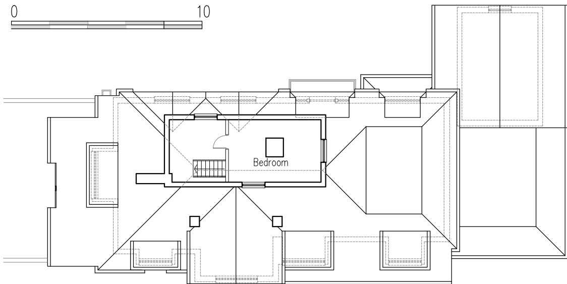
1:200 Existing Second floor plan
