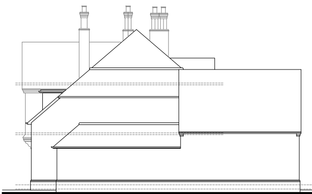
1:200 Existing Rh side Elevation
