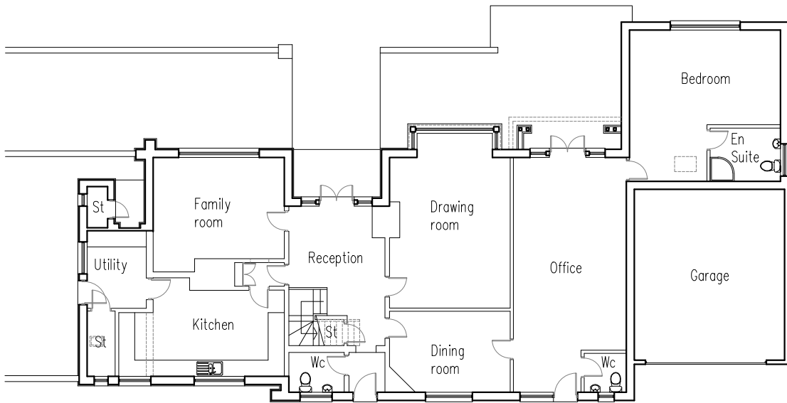
1:200 Existing Ground floor plan
