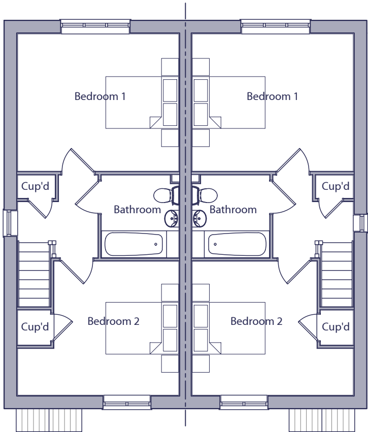
FIRST FLOOR PLAN PLOT 4009 PLOT 4008
