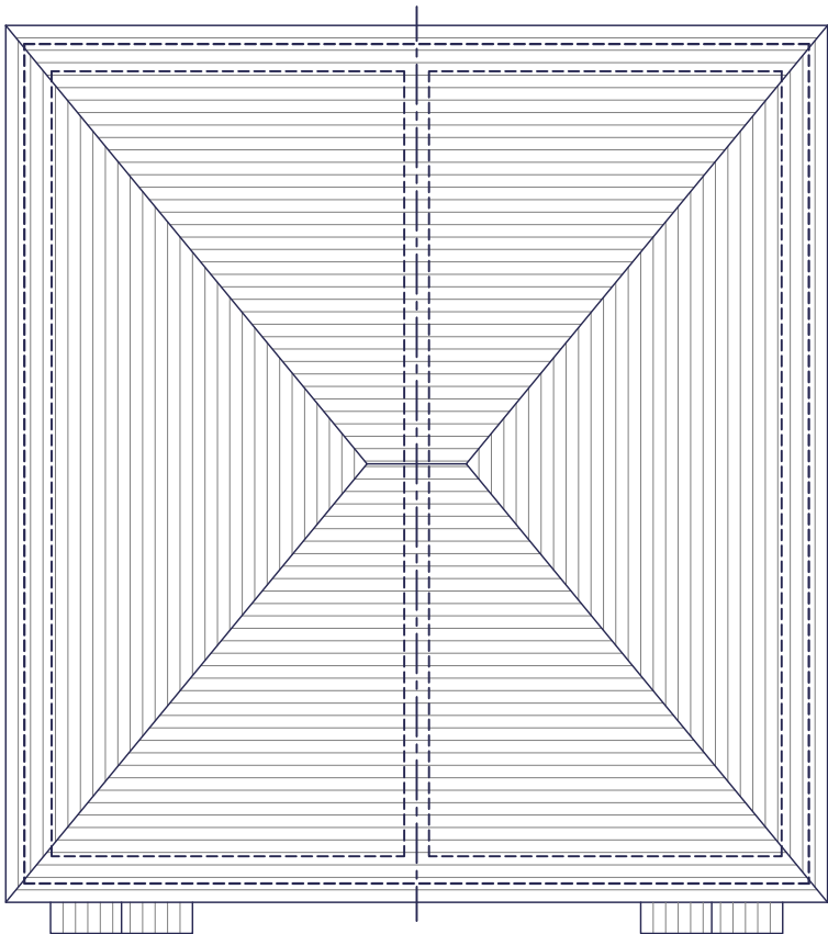
ROOF PLAN PLOT 4009 PLOT 4008
