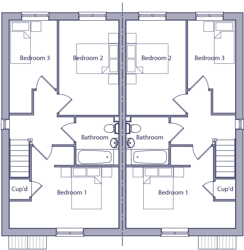
FIRST FLOOR PLAN PLOTS 3060, 4023, 4097 & 4099
