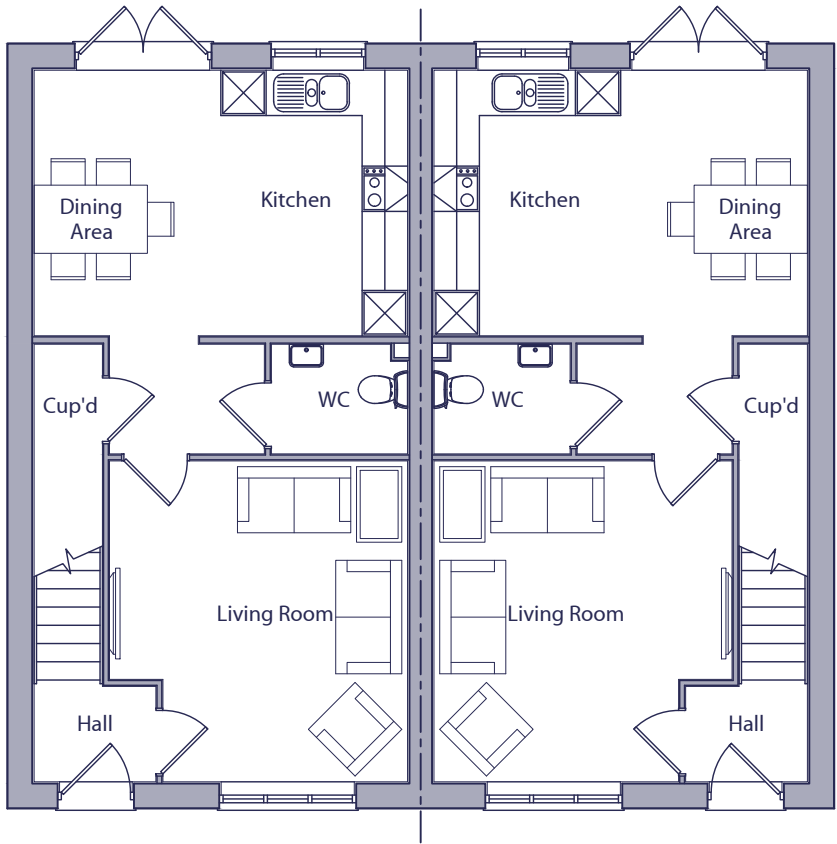
GROUND FLOOR PLAN PLOTS 3060, 4023, 4097 & 4099
