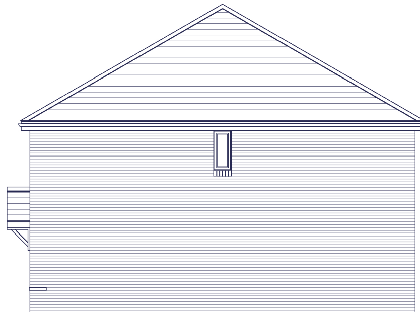
SIDE ELEVATION PLOTS 3061, 4022, 4096 & 4098.
