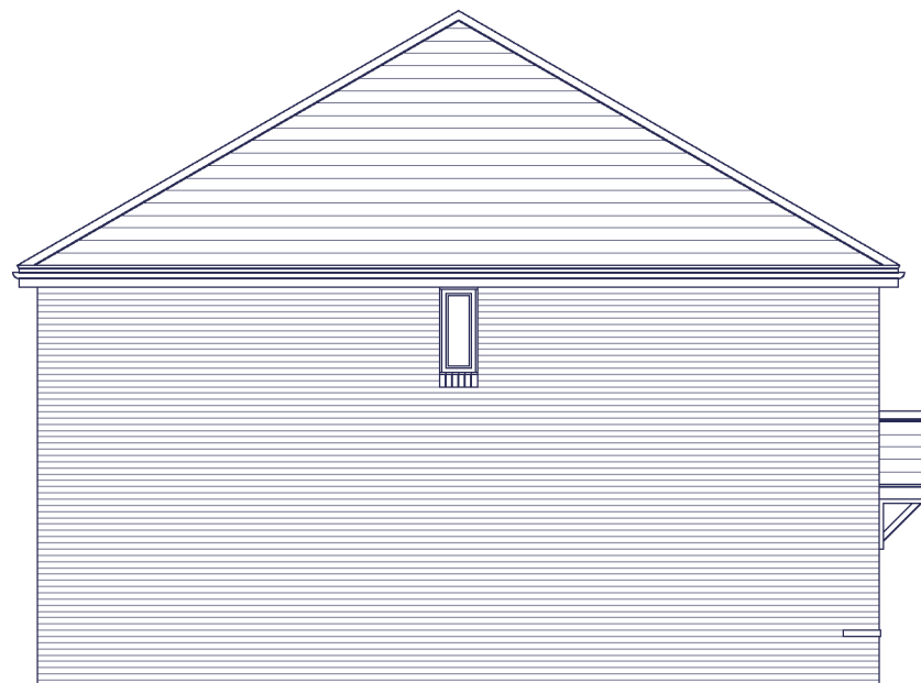
SIDE ELEVATION PLOTS 3060, 4023, 4097 & 4099
