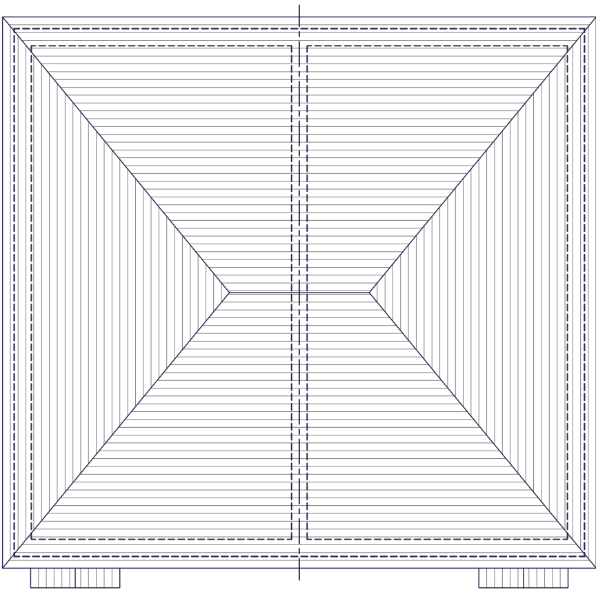
ROOF PLAN PLOT 3091 PLOT 3092
