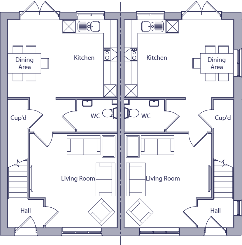
GROUND FLOOR PLAN PLOT 3091 PLOT 3092
