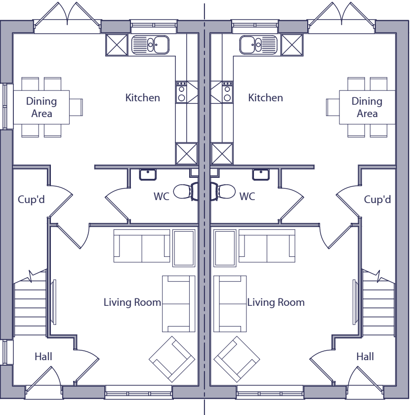
GROUND FLOOR PLAN PLOT 4005 PLOT 4004
