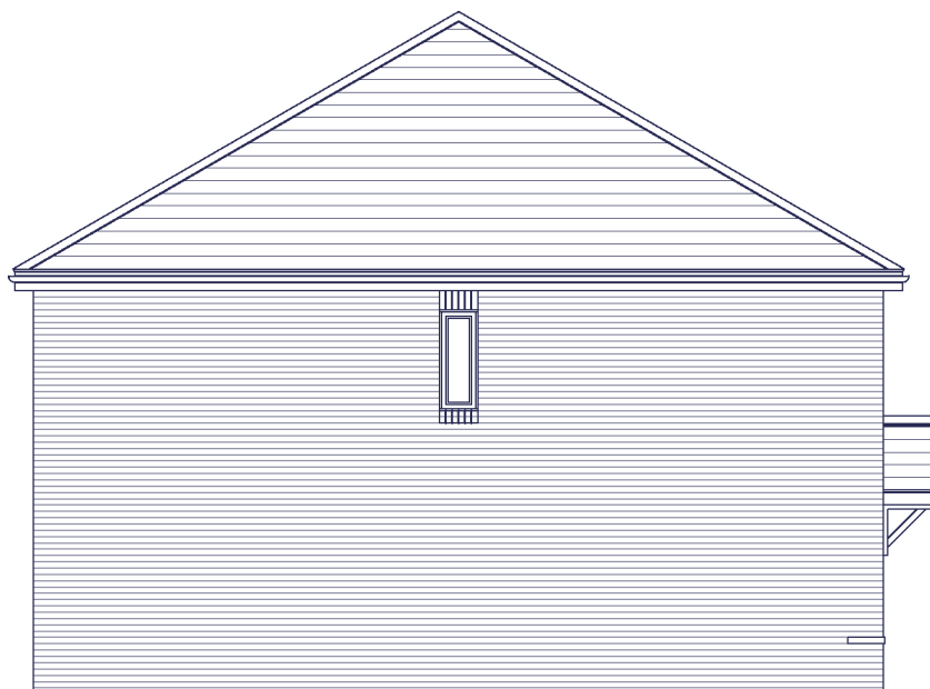
SIDE ELEVATION AL41 TYPE - PLOT 3098
