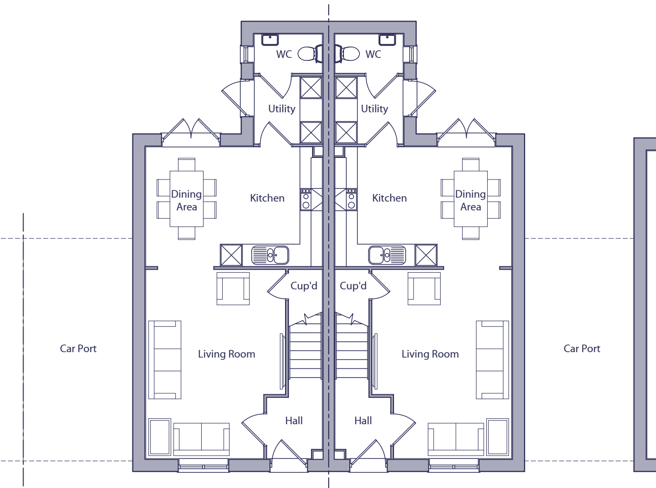
GROUND FLOOR PLAN PLOT 4012
