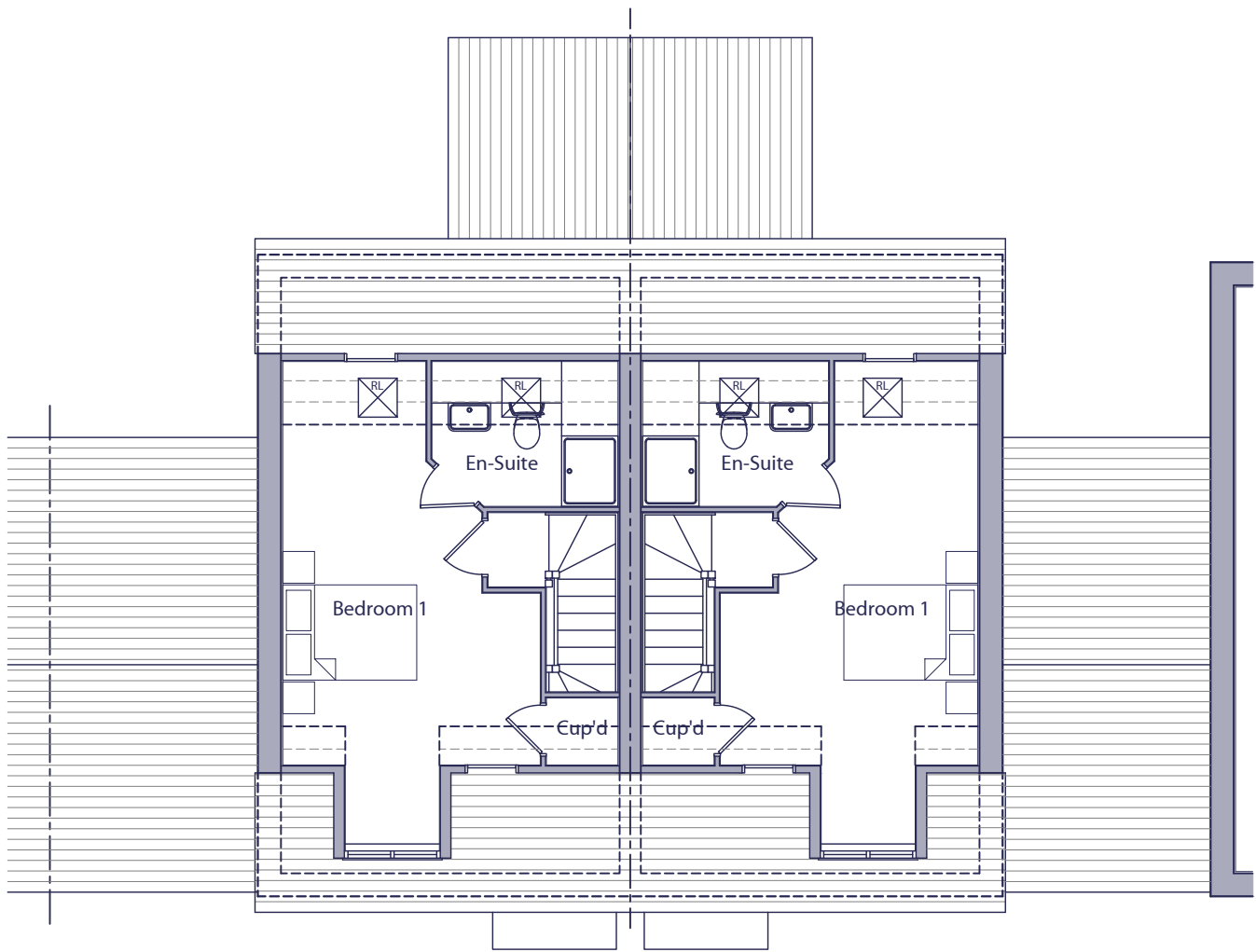
SECOND FLOOR PLAN PLOT 4012
