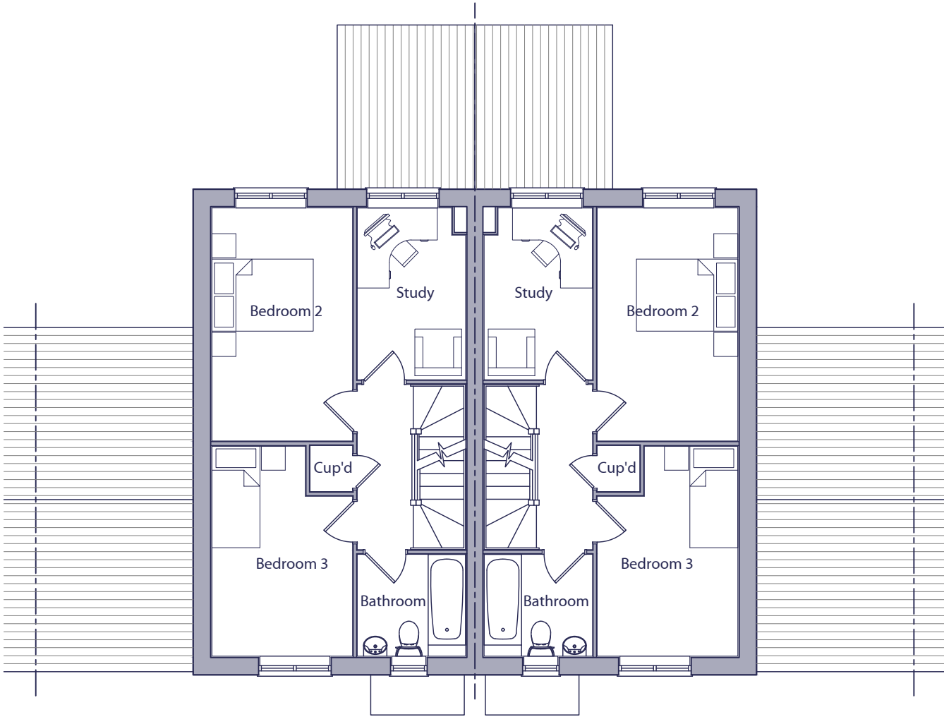
FIRST FLOOR PLAN PLOT 4014
