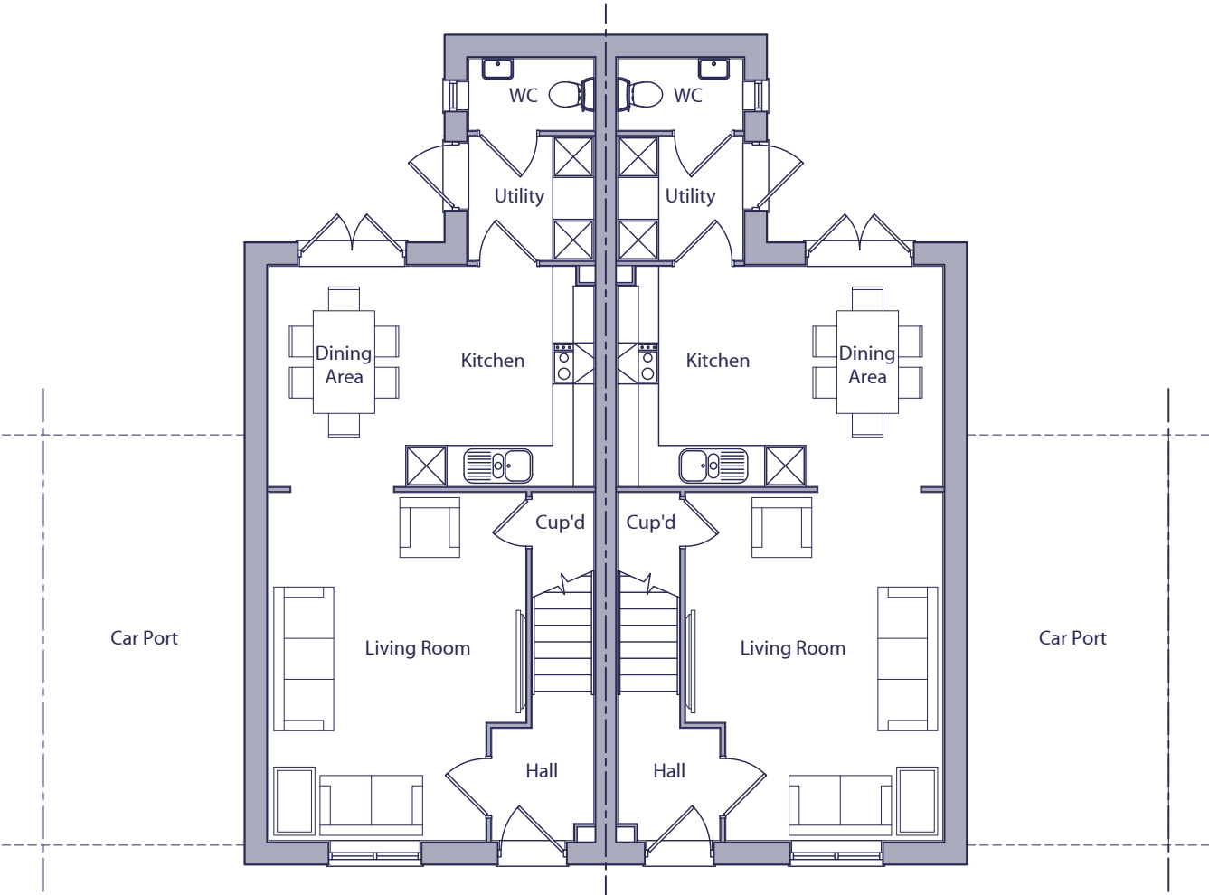
GROUND FLOOR PLAN PLOT 4014
