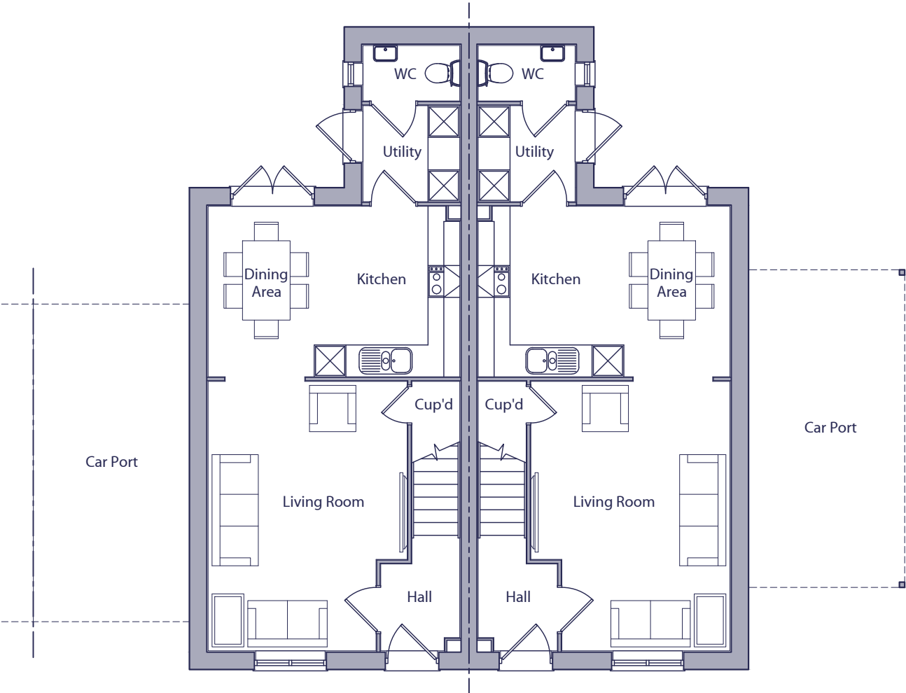
GROUND FLOOR PLAN PLOT 4031
