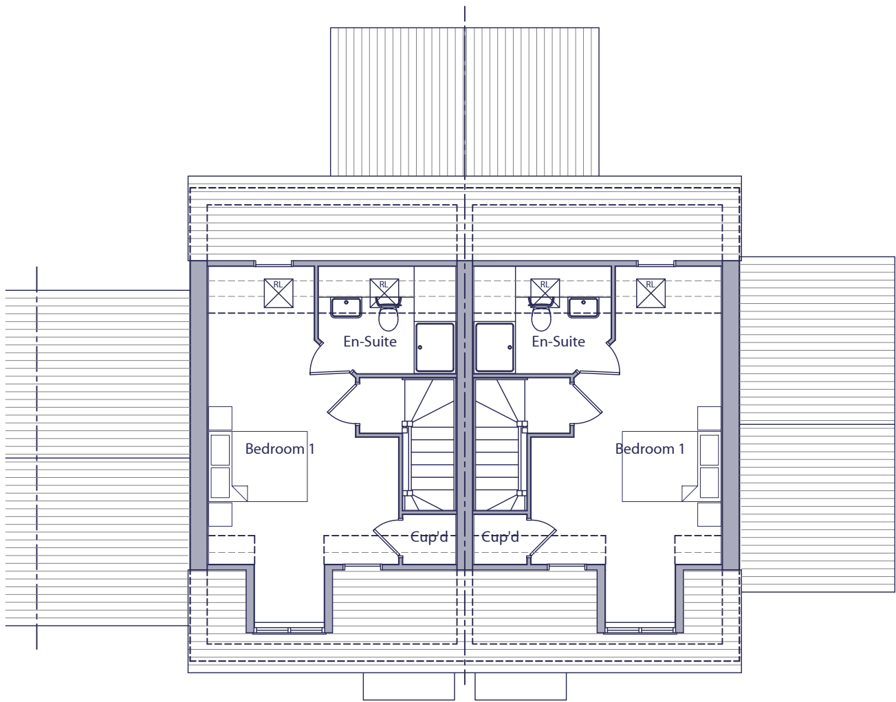
SECOND FLOOR PLAN PLOT 4031
