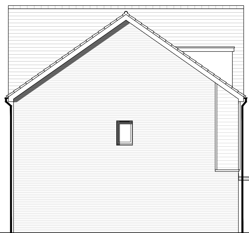
Side Elevation
