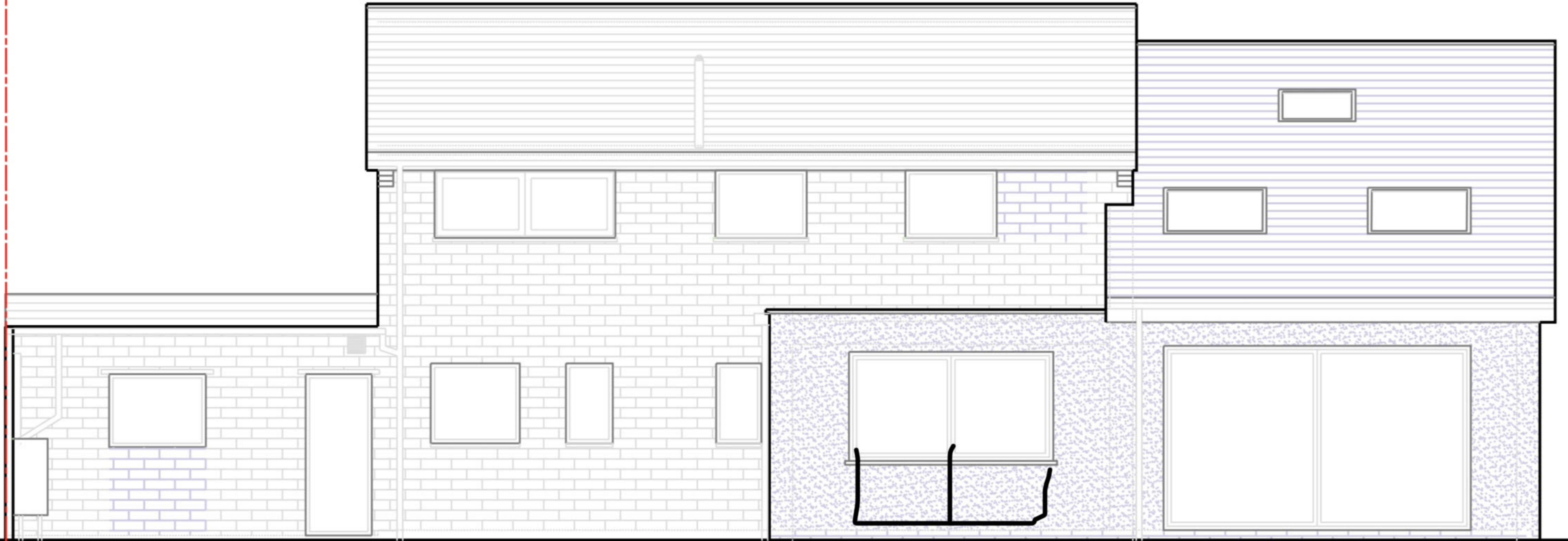
PROPOSED REAR ELEVATION
