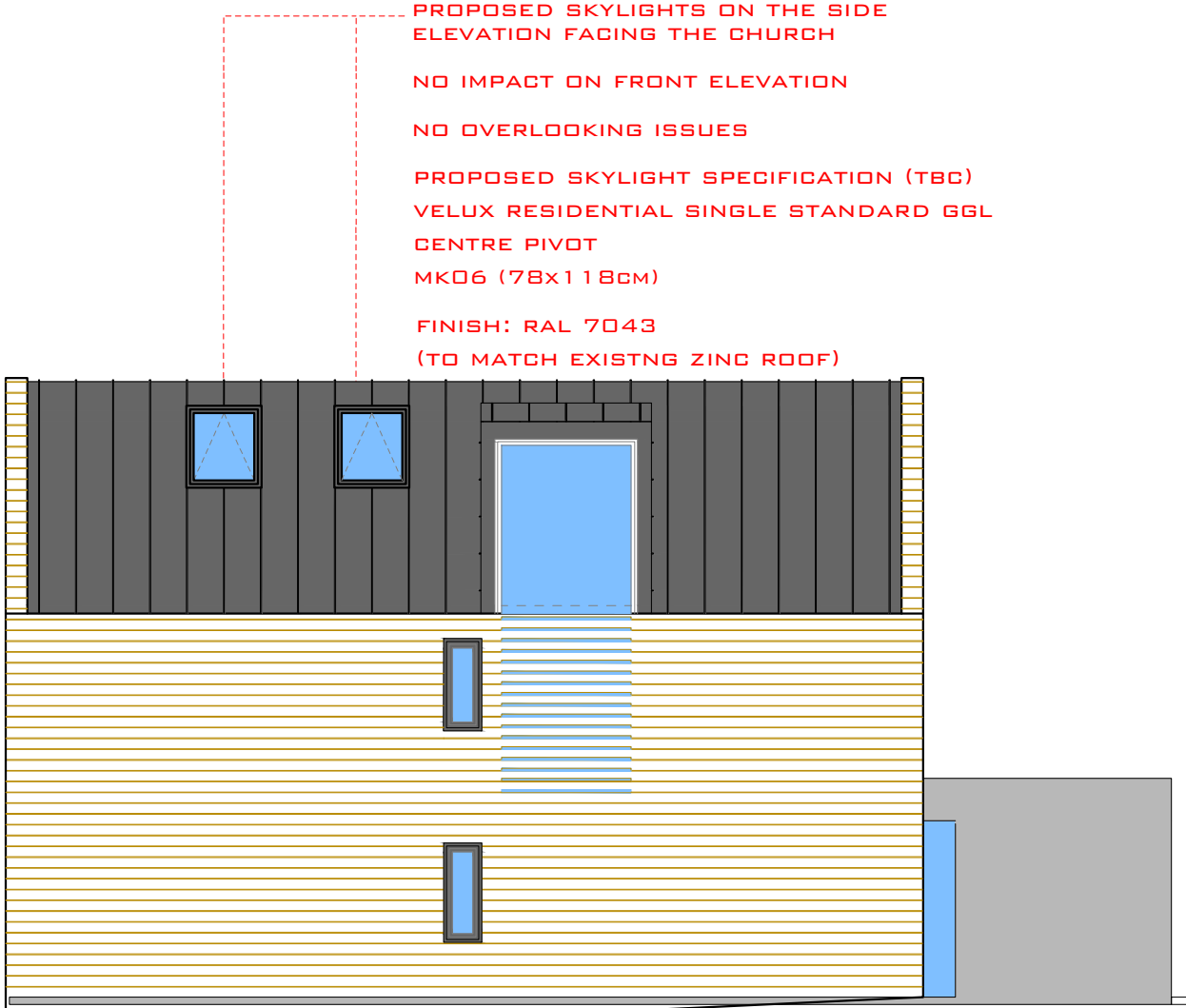
SIDE ELEVATION (FACING CHURCH) PROPOSED
