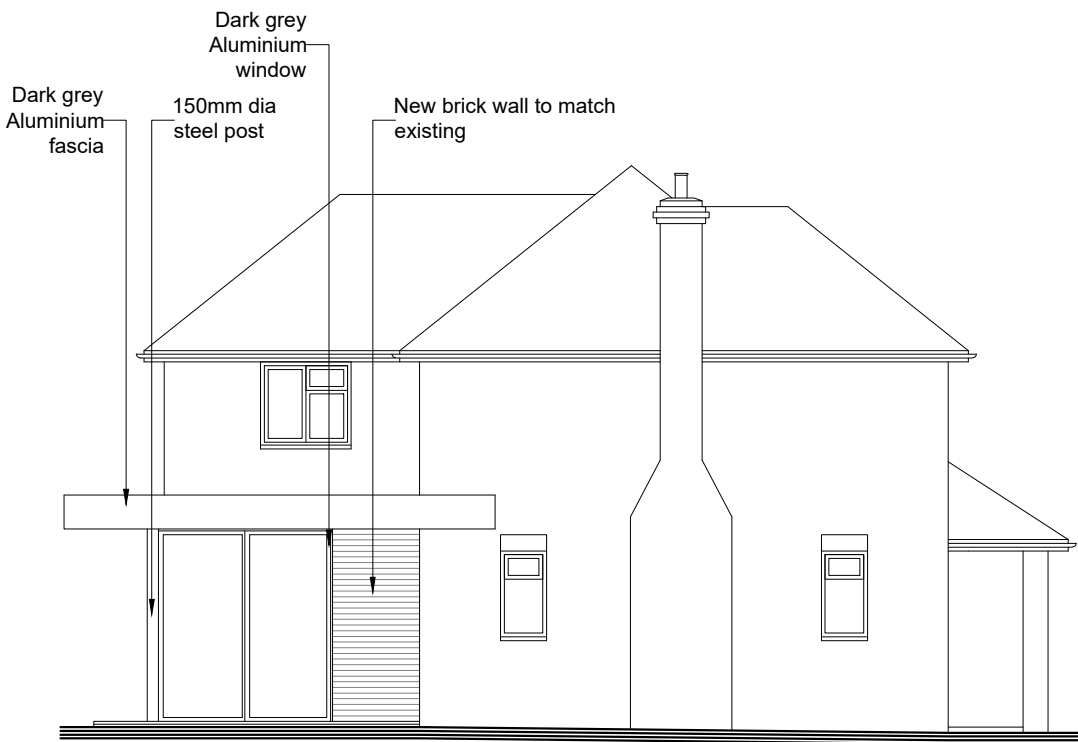
1:100 Proposed Rh side Elevation
