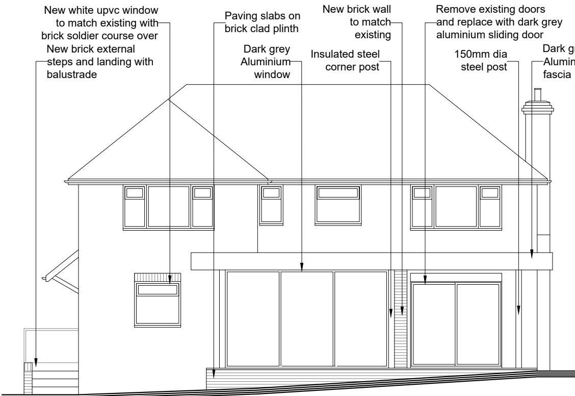
1:100 Proposed Rear Elevation
