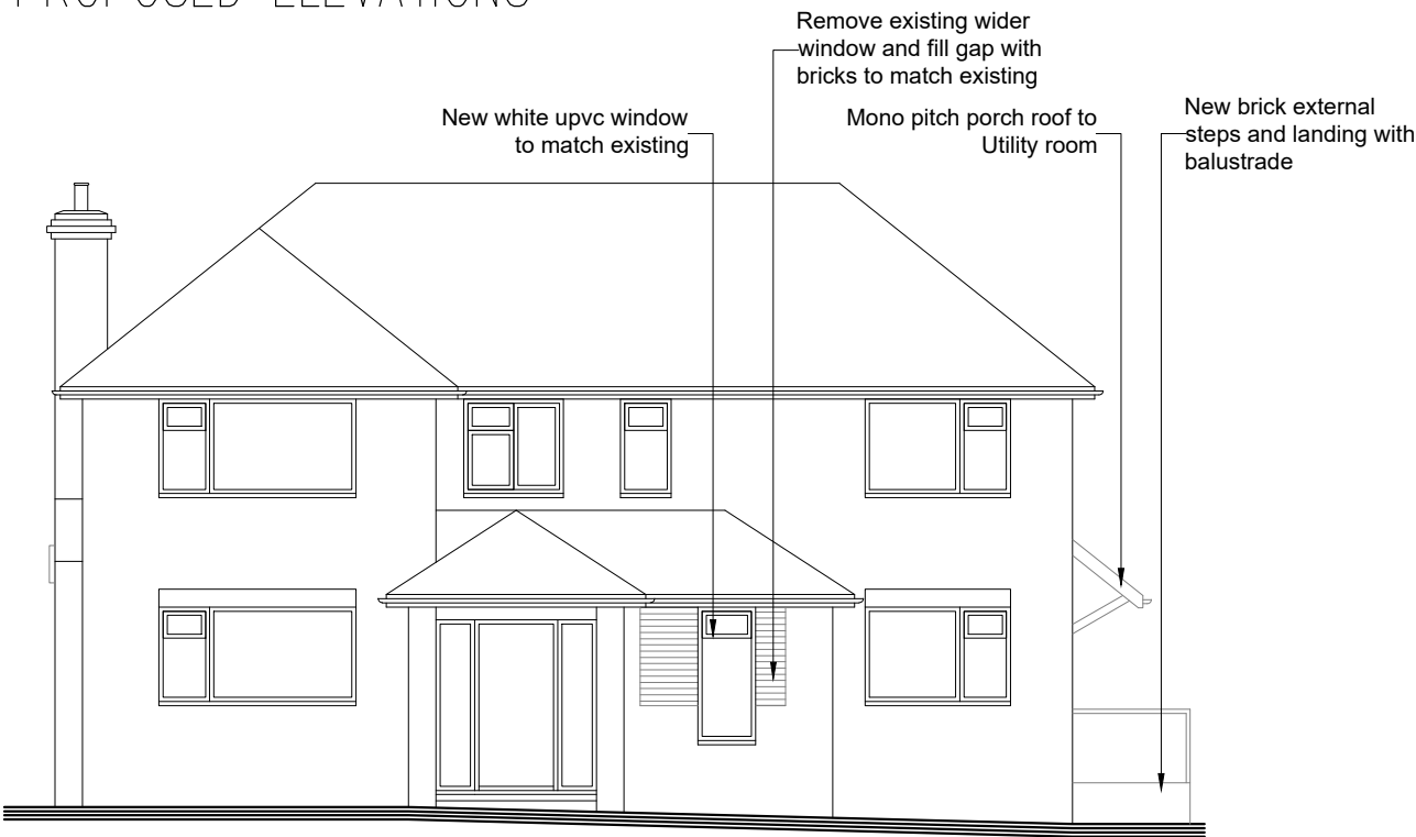
1:100 Proposed Front Elevation
