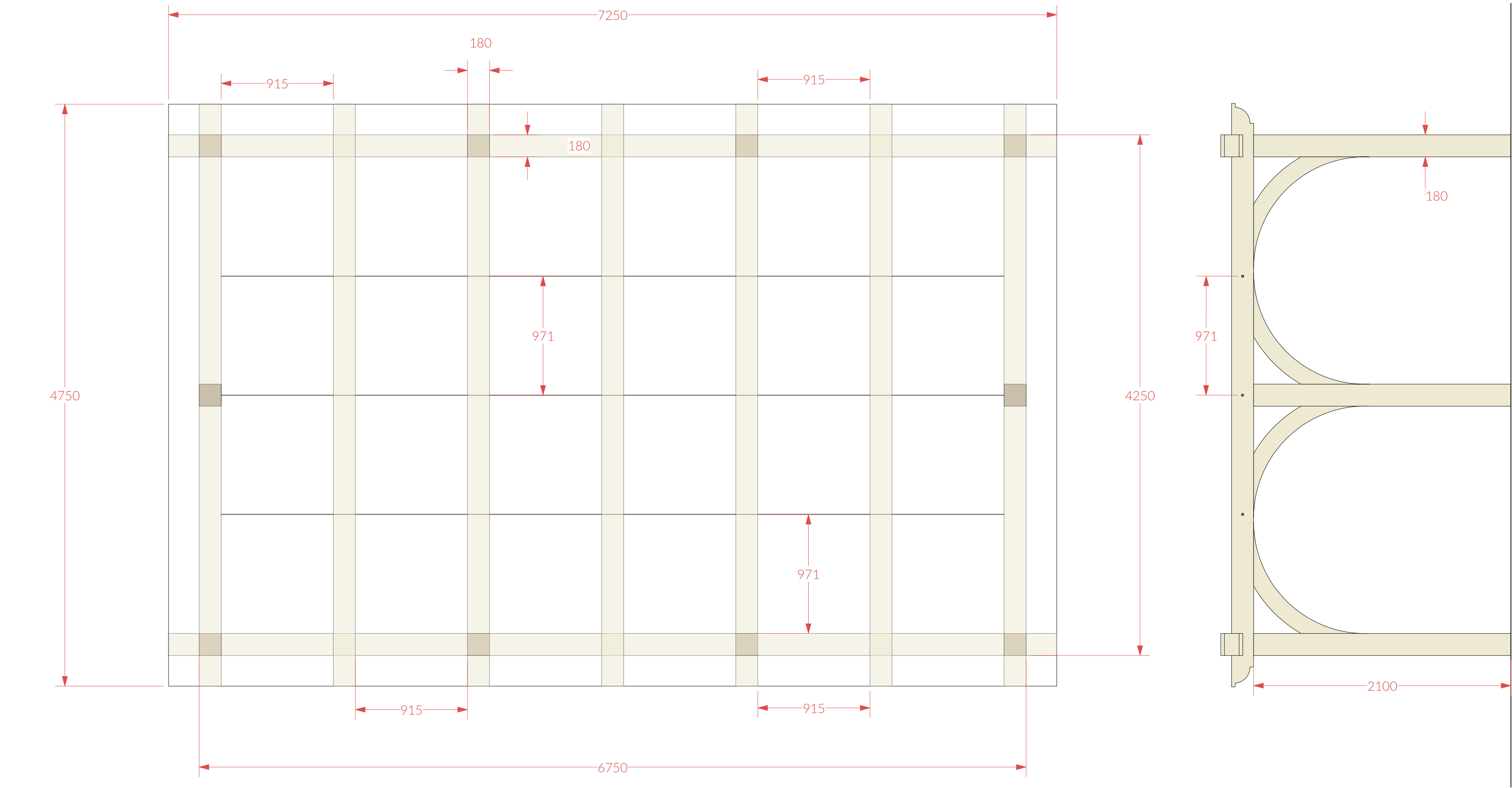
1 Plan view
