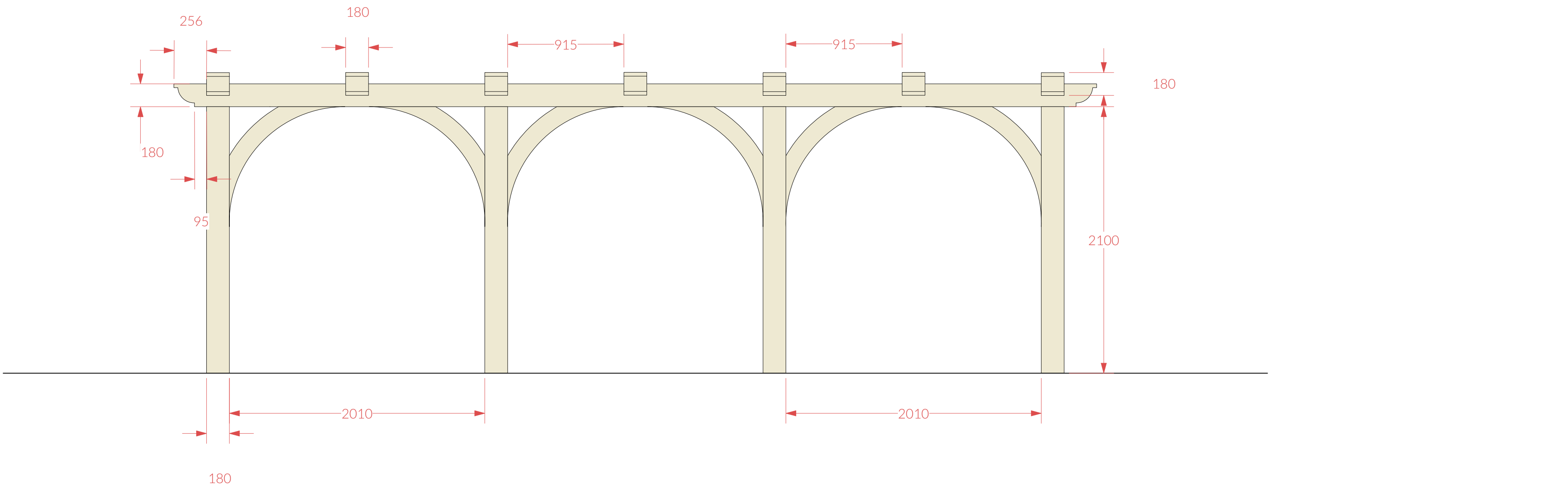
3 Side elevations
