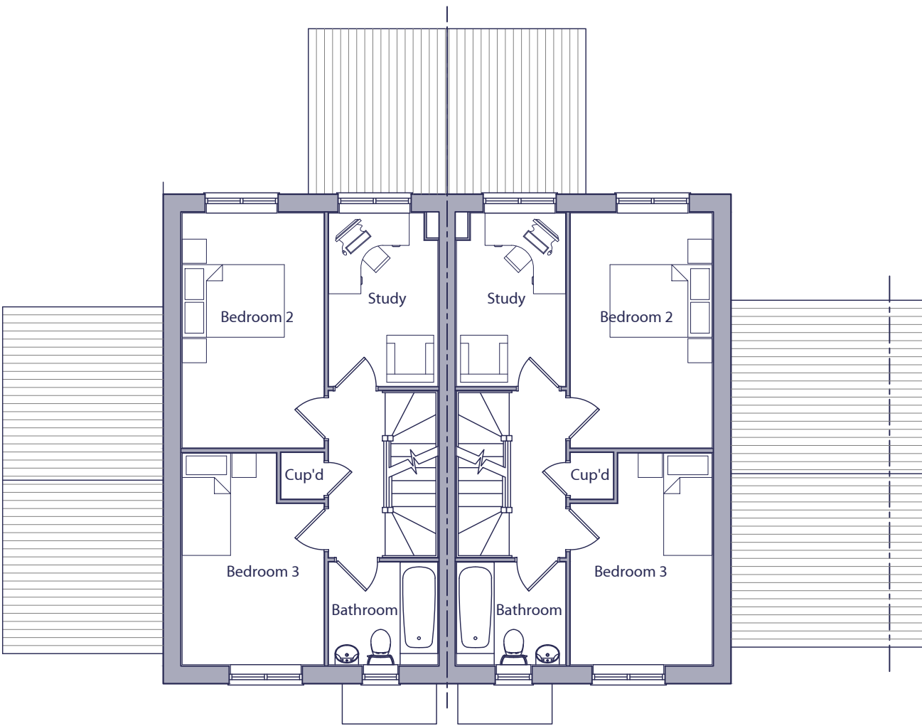
FIRST FLOOR PLAN PLOT 4042
