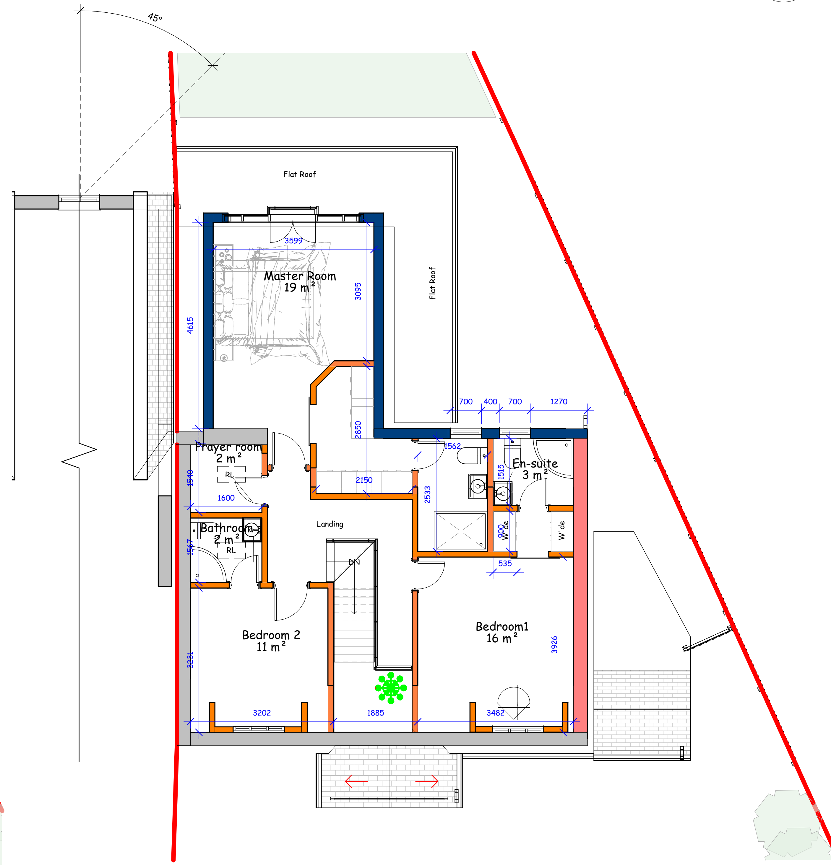
Proposed First Floor 1 : 50
