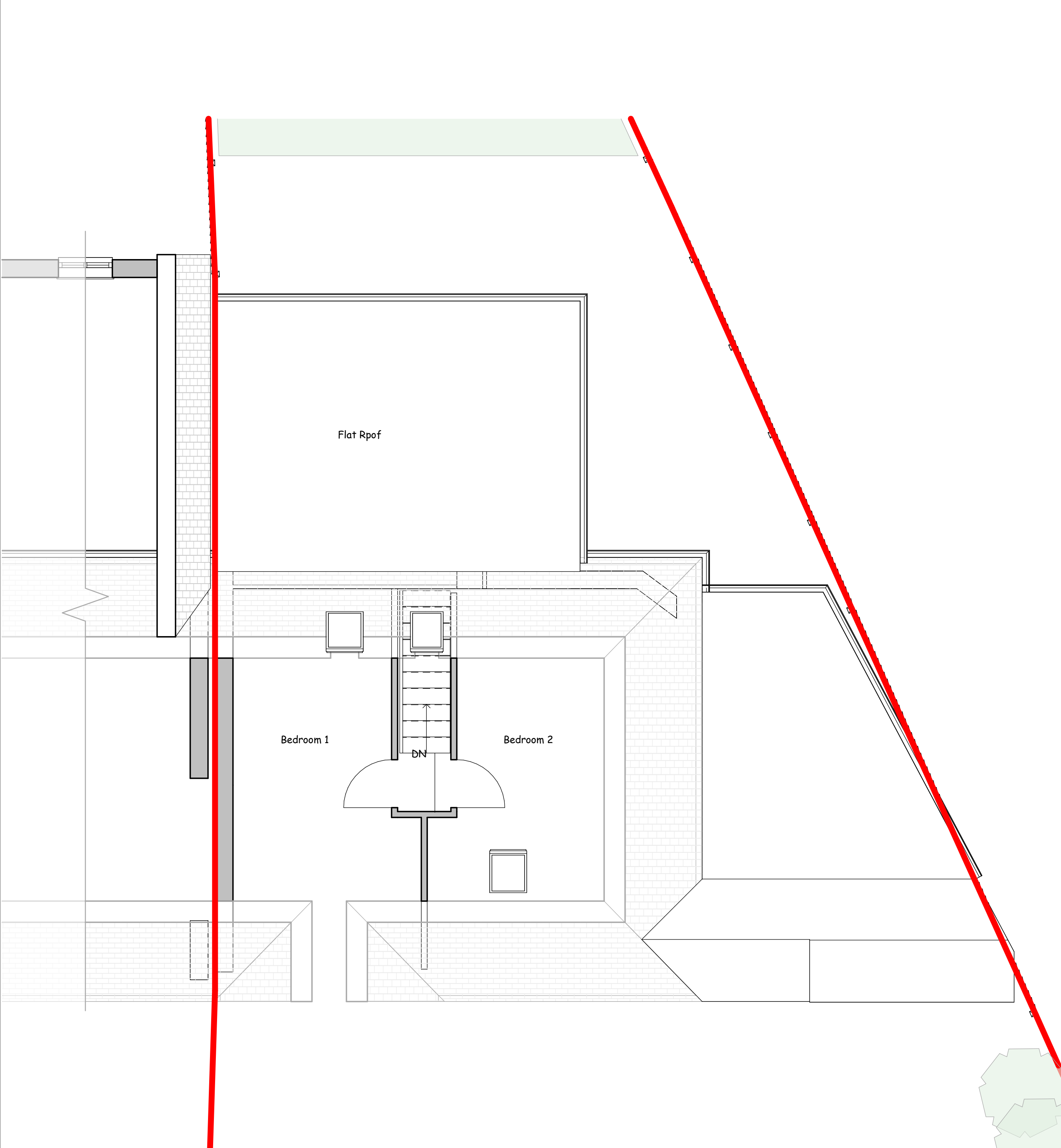
Existing First Floor 1 : 50
